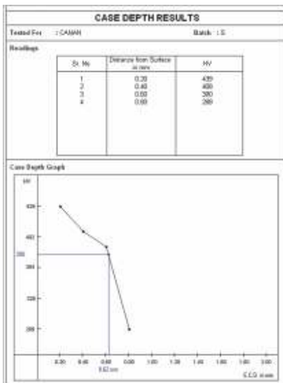
Case Depth Results
